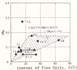
Fig. 28 : S-D R_l Relationship
